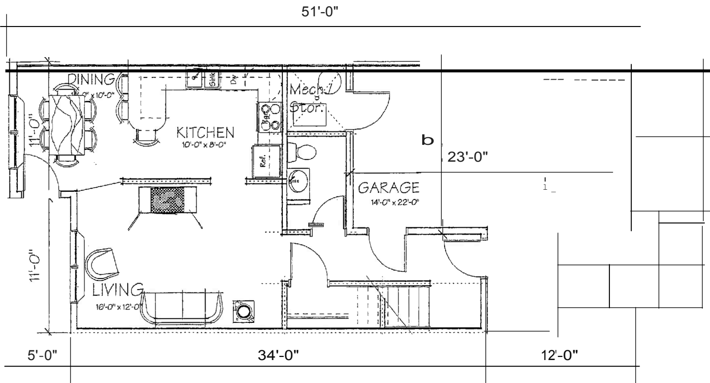
ain Floor
