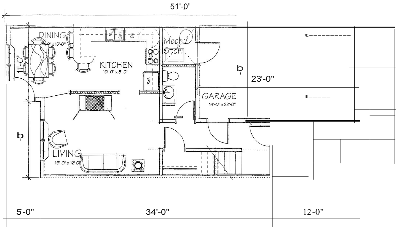
Main Floor 625sF
